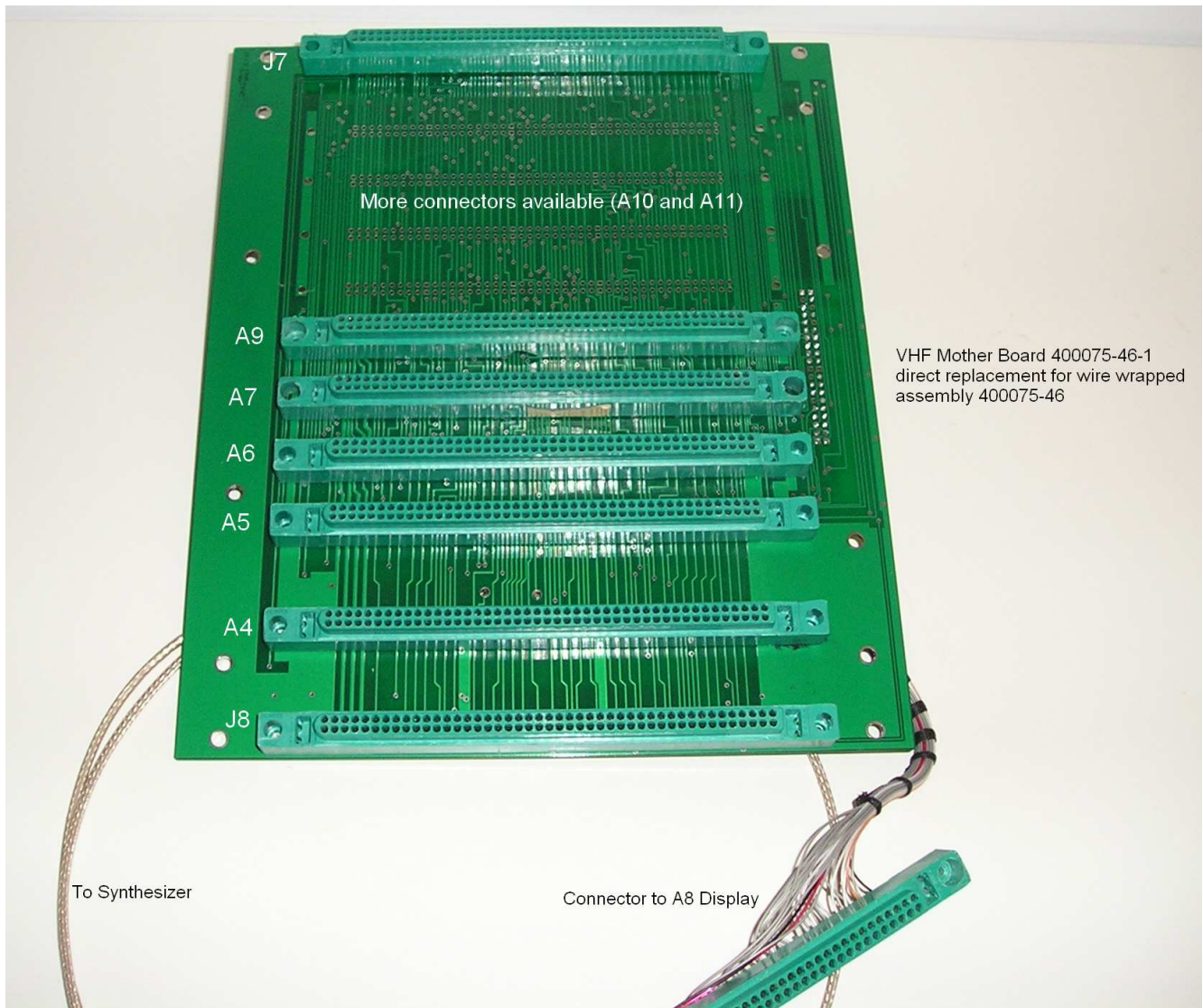
Fig.1 DF2100 VHF Receiver Mother Board 400075-46
